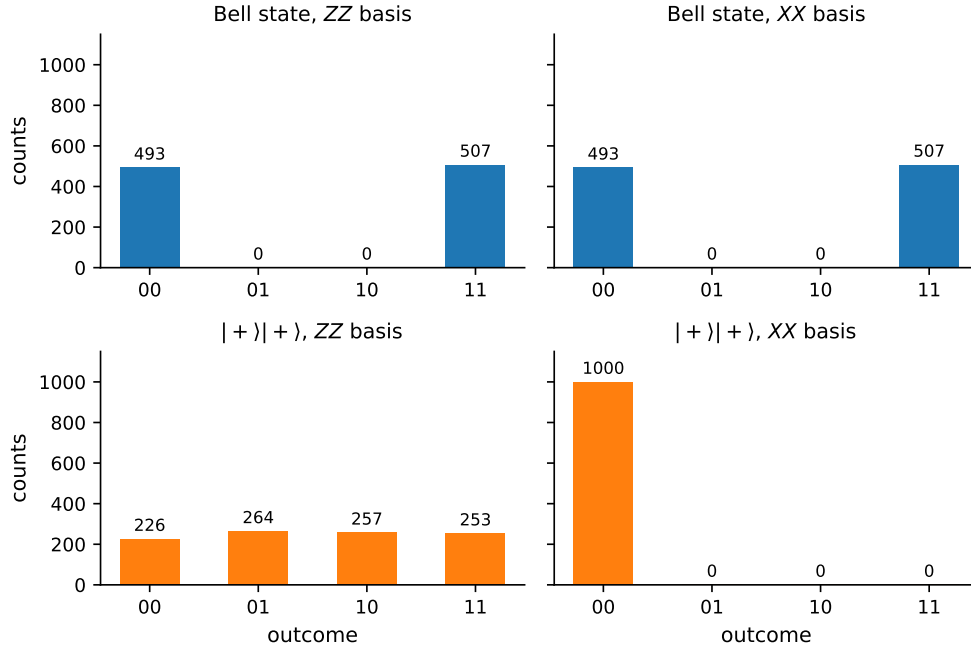
Figure 5: Both qubits measured in the Z basis (left) and the X basis (right), 1000 shots each. Top: the Bell state, correlated in both. Bottom: the product state |++\rangle , correlated in X only.
